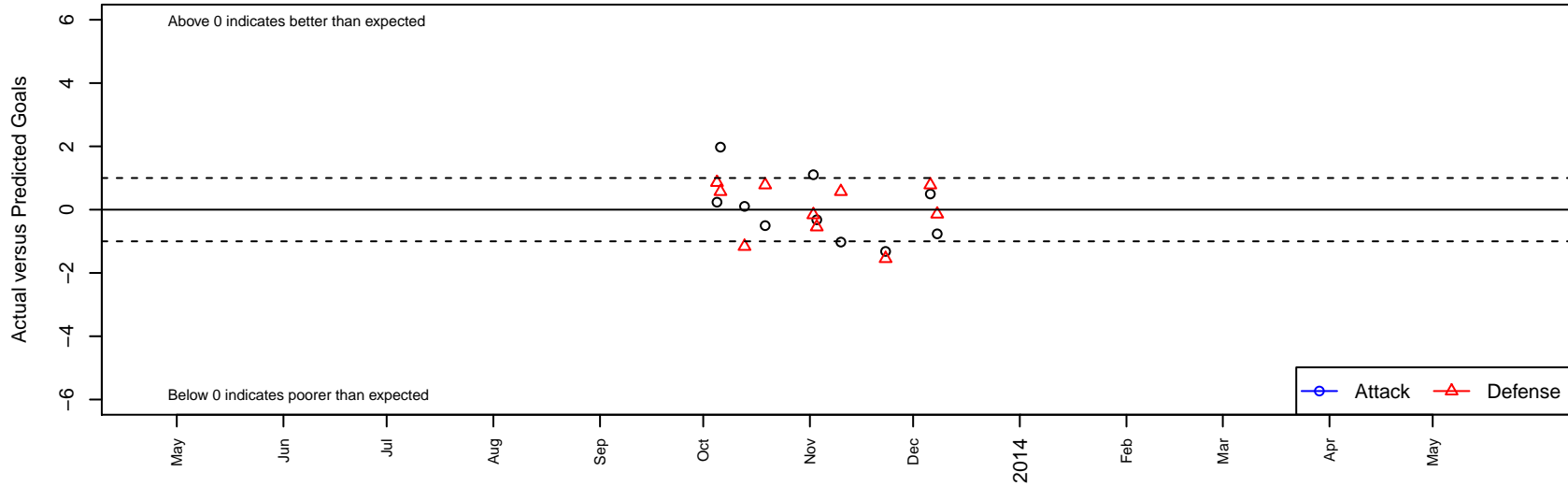
Davis Legacy 01 Dynamite G00 Dots are actual minus expected GF (blue circles) and GA (red triangles). Blue line is smoothed change in attack strength. Red is smoothed change in defense strength.
